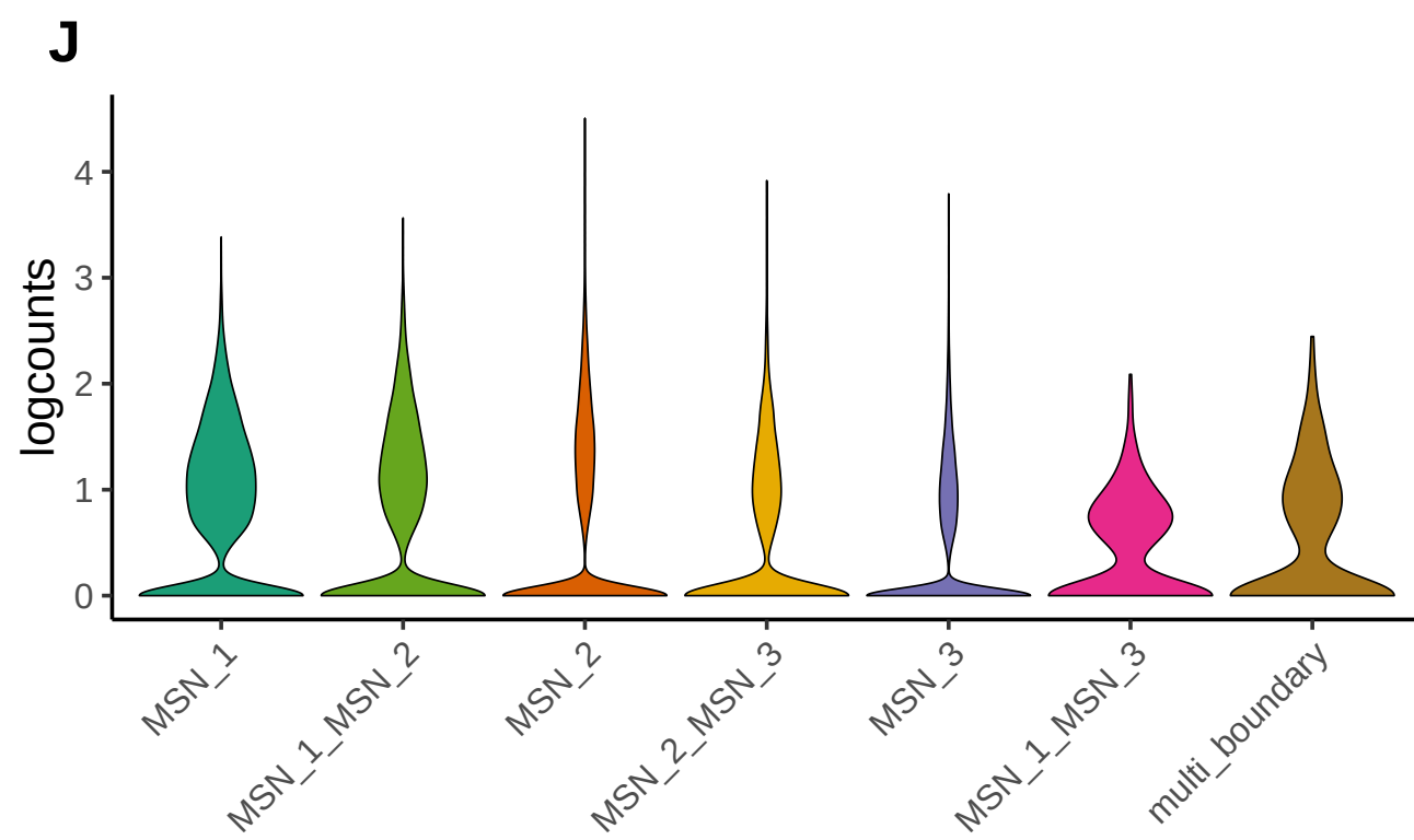
PDE10A
