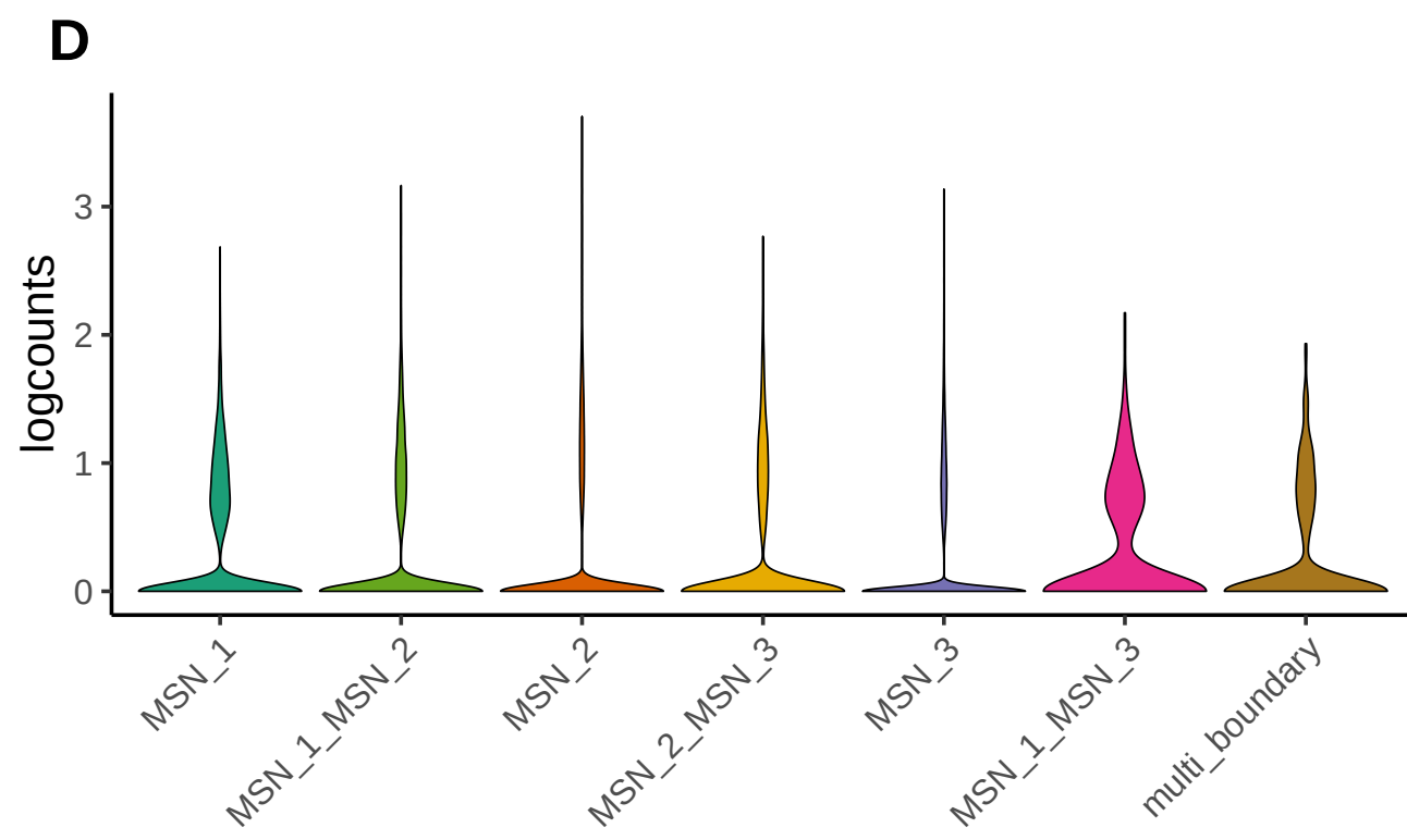
CARTPT
