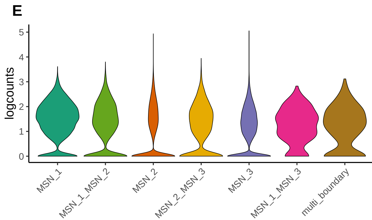
TAC1
