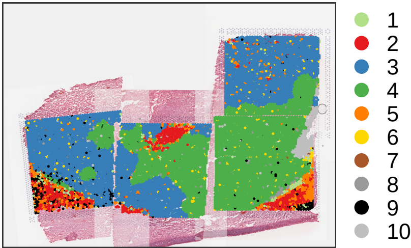
Random start: 1
