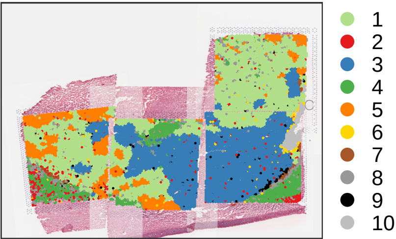
Random start: 2
