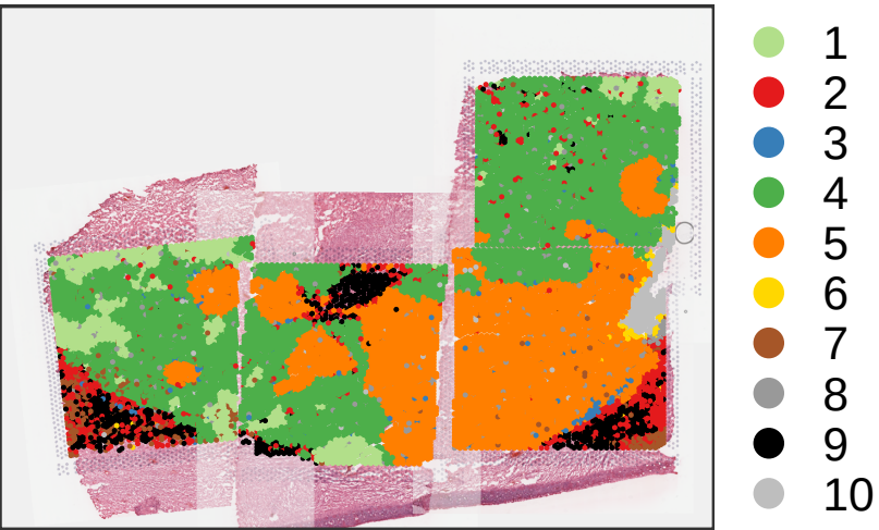
Random start: 3
