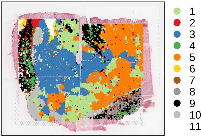
Random start: 2
