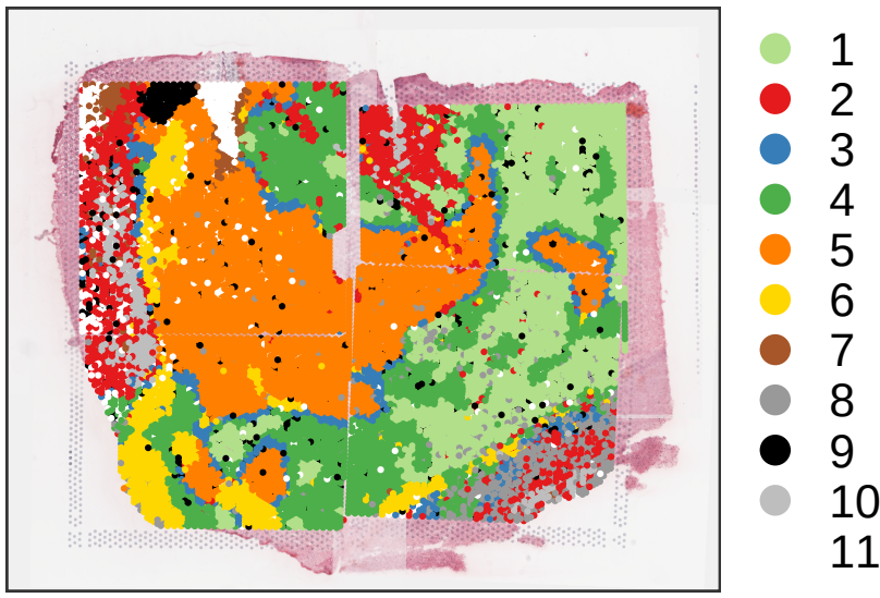
Random start: 3
