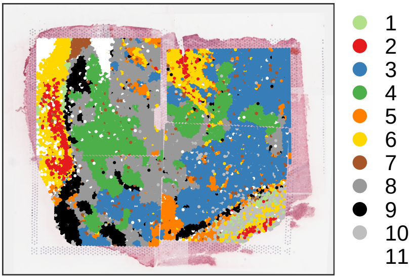
Random start: 1
