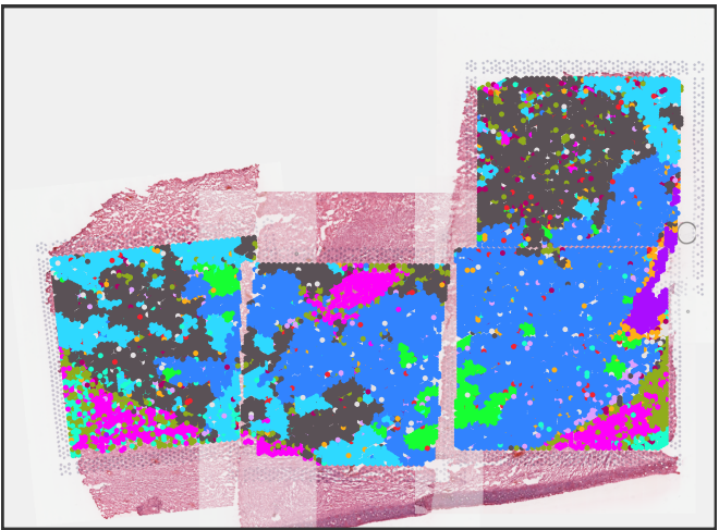
Random start: 2
