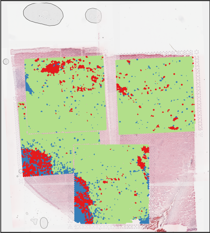
Random start: 1
