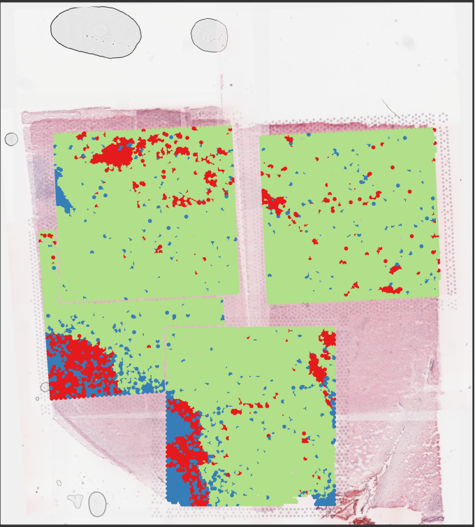
Random start: 2
