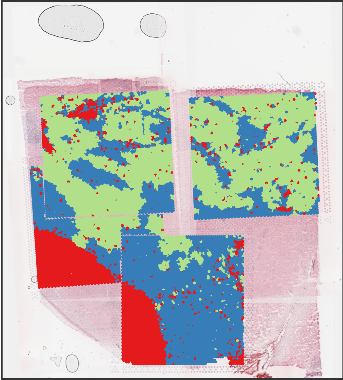
Random start: 3
