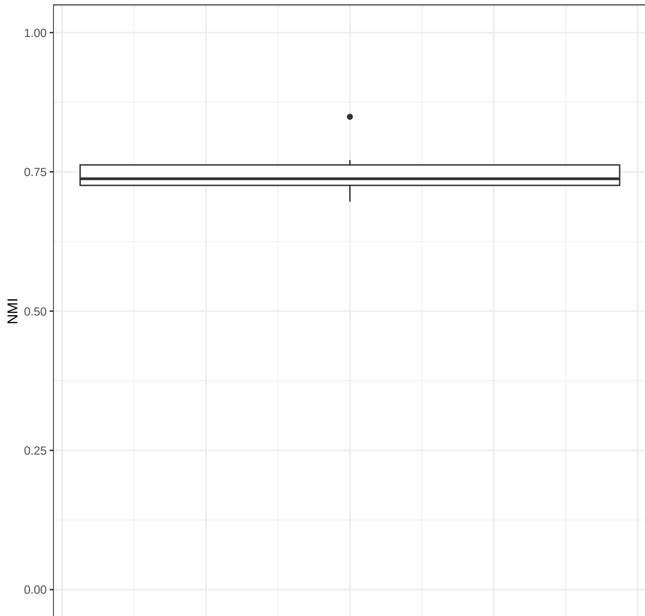
Accuracy of PRECAST Leave-One-Out Cross-Validation
