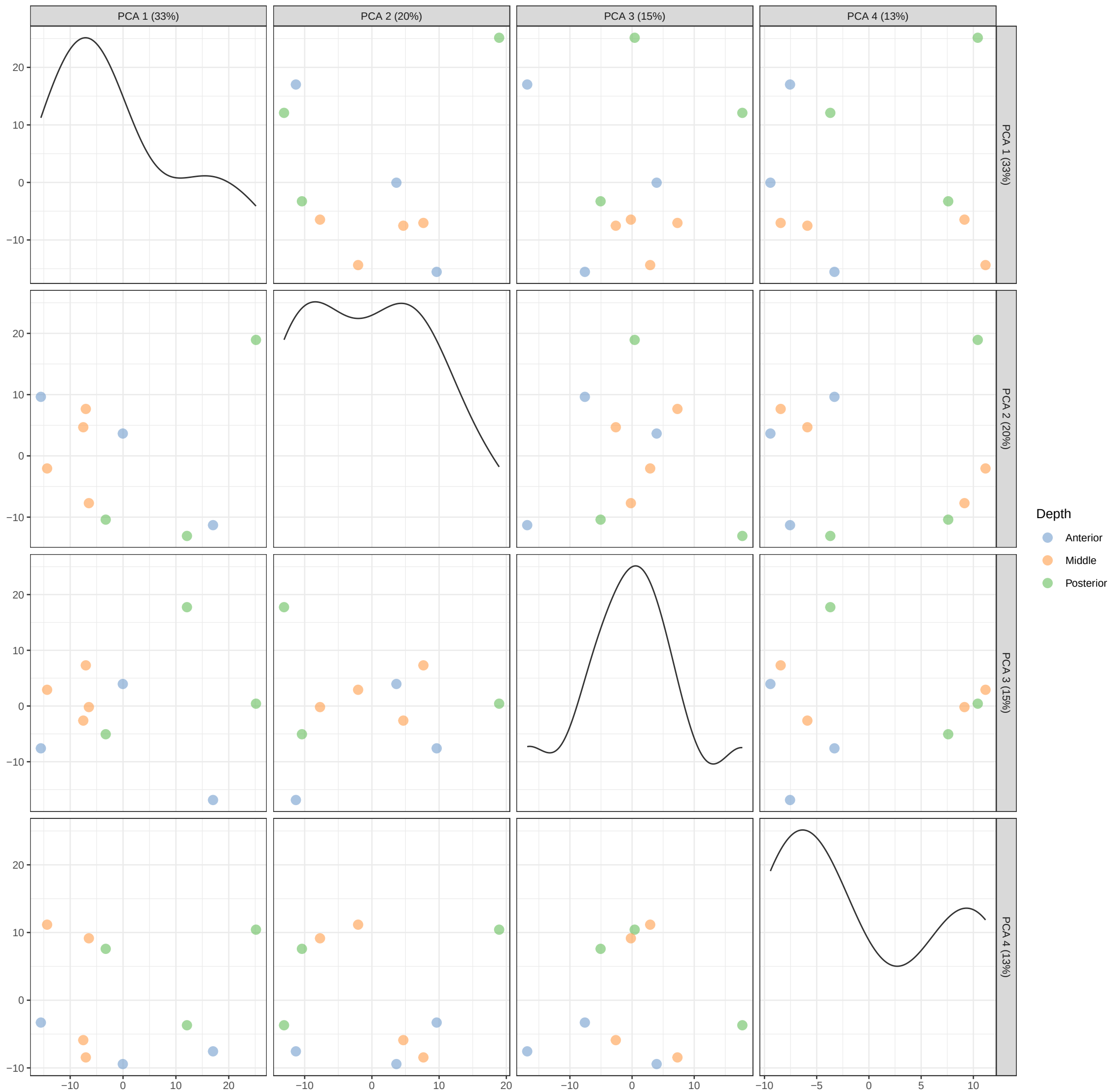
DRD1_MSN_A
