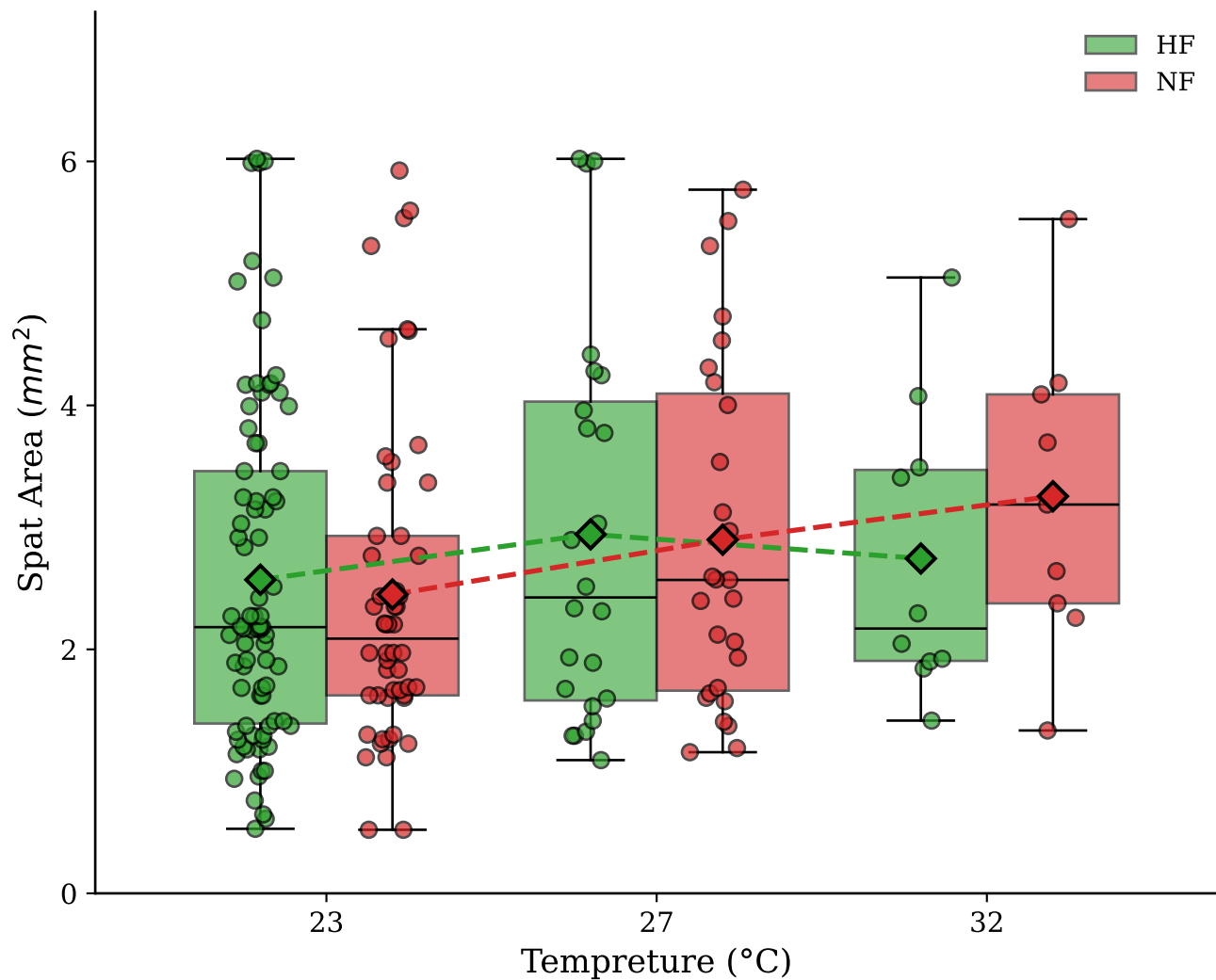
Size distribution of settled spats by Temperature and morph
