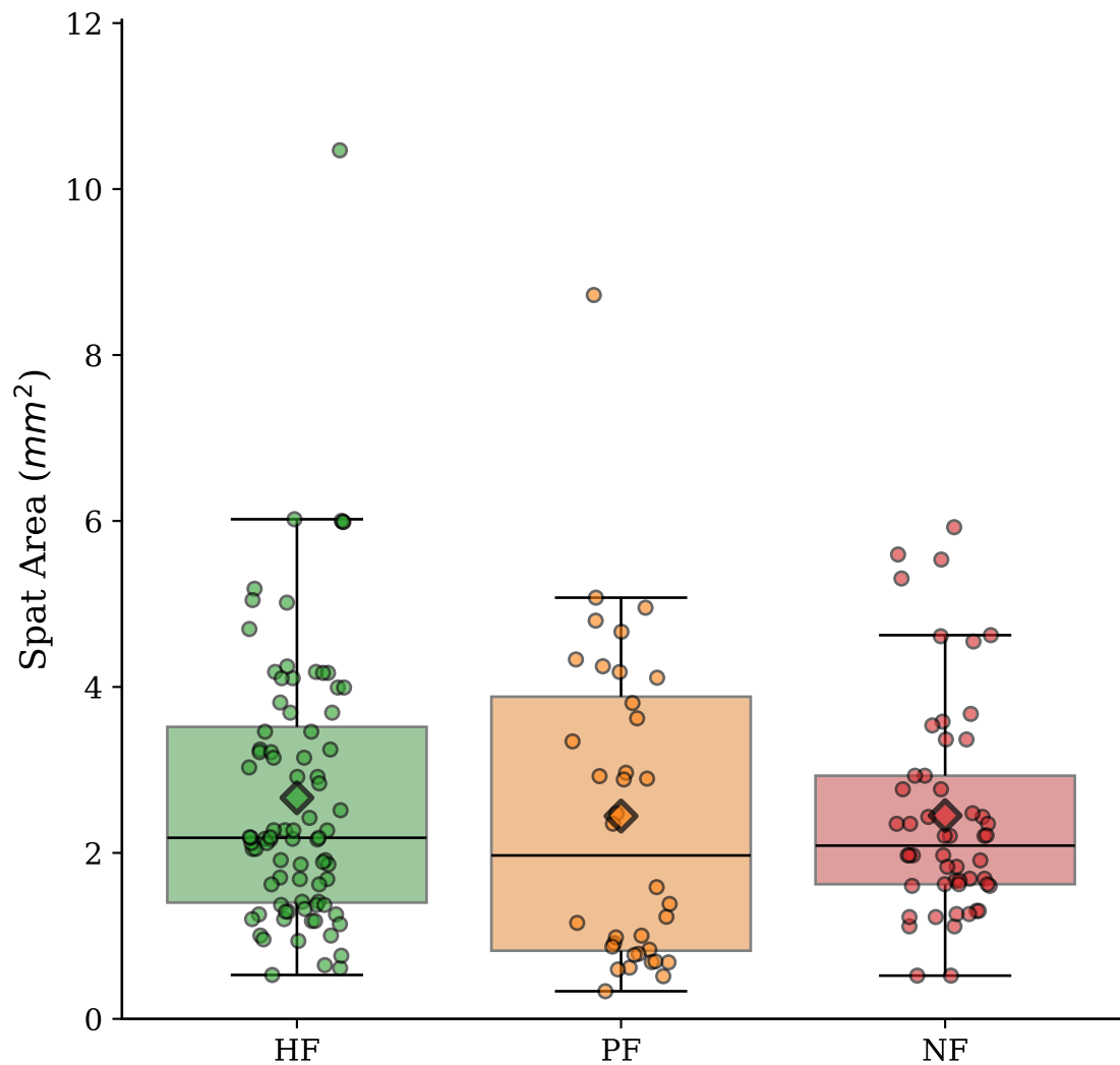
Size distribution of settled spats from diffrrent morphs
