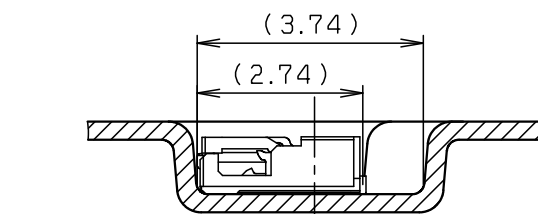
SECT. F-F (S=8:1) (10~49P)
