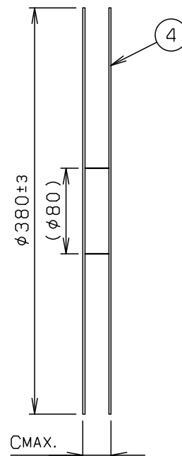
SECT. E-E (51~61P)
