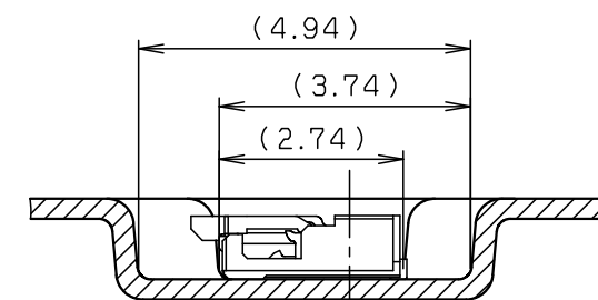
SECT. F-F (S=8:1) (10~49P)
