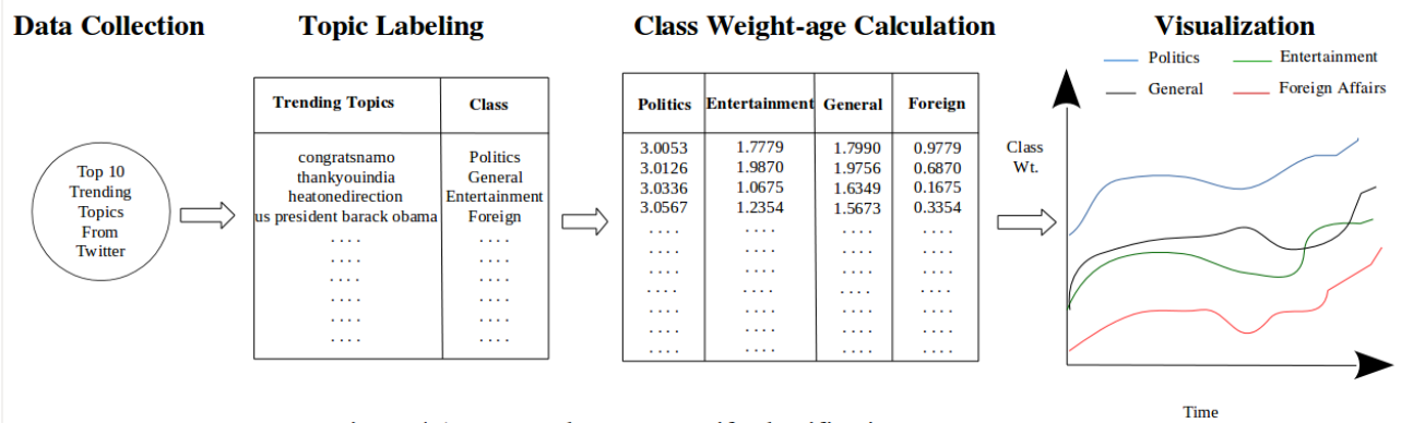
Figure 4.1. Proposed Concept-Drift Identification System
