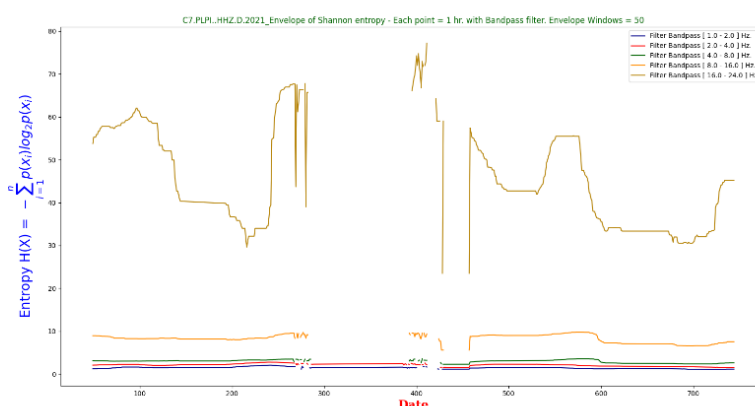
Fig. 86 Volcano and effusive eruption type. Graph (lines) comparing envelopes using the 5 sets of bandpass filter values, using a time interval (Julian days 274-304), equivalent to October 2021.
