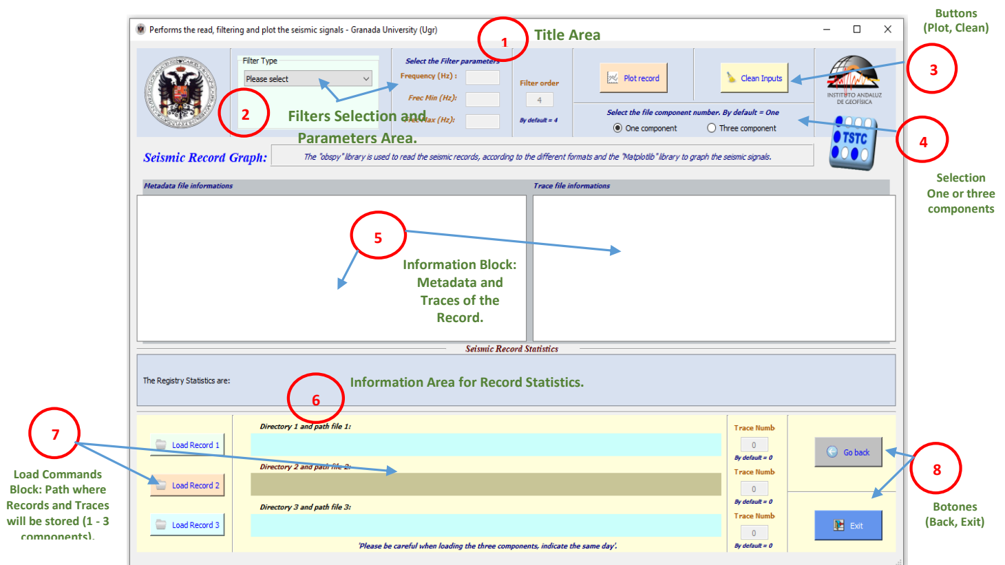
Fig. 7 Interface of the Module for Reading, Filtering, and Plotting Records and its Components.
