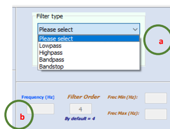
Fig. 36 Upper Part -> (a) Filter Type Selection ( Lowpass , Highpass , Bandpass , Bandstop ). Lower Part -> (b) Filter Parameters ( Frequency , Filter Order , Minimum Frequency , Maximum Frequency ).
