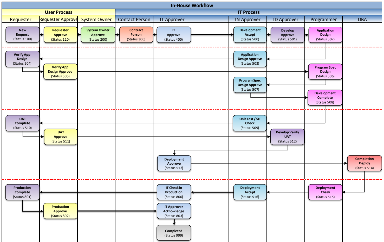
Development Workflow Diagram
