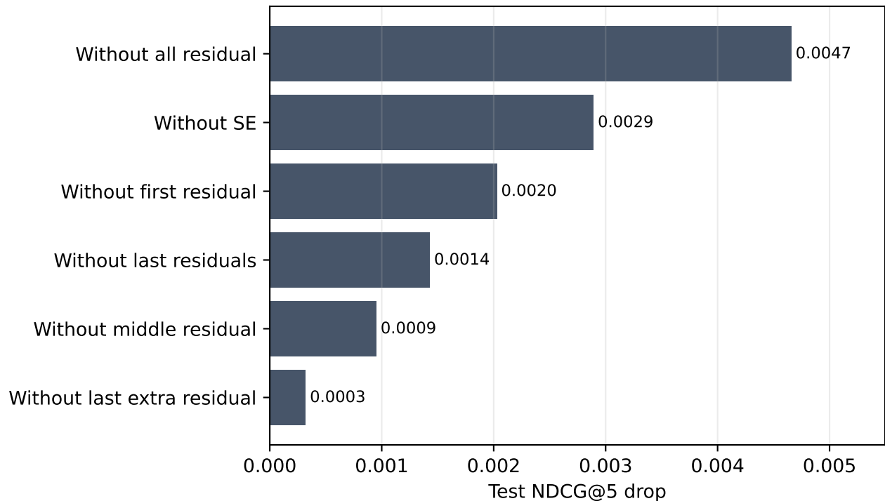
(c) Test NDCG@5 drop from full TitLeNet
