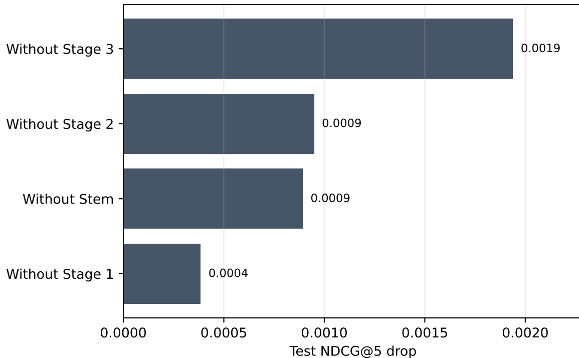
(c) Test NDCG@5 drop from full TitLeNet
