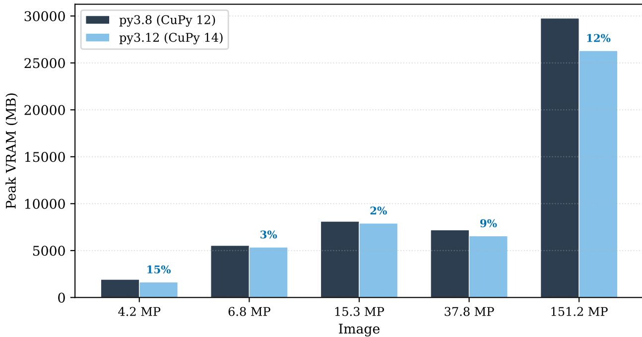
Peak GPU memory: py3.8 vs py3.12 (A100-SXM4-80GB)
