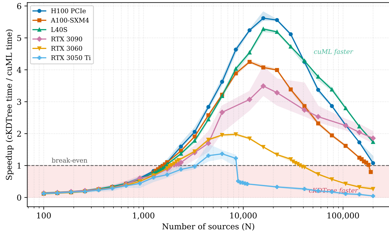
cuML vs cKDTree crossmatch: synthetic benchmark
