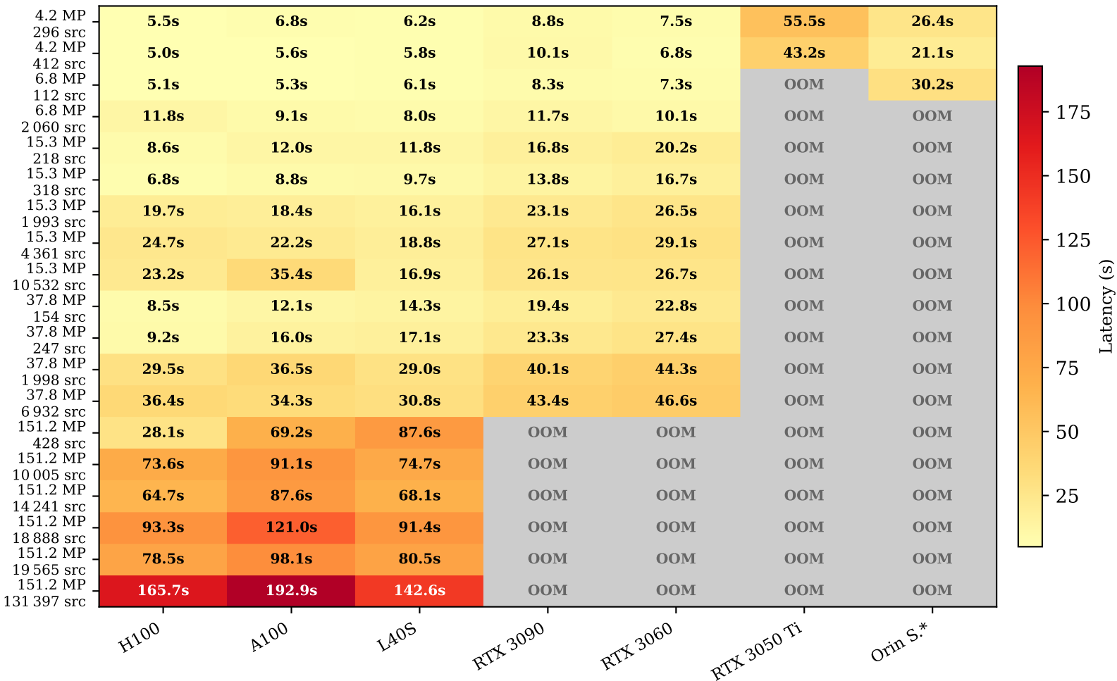
End-to-end latency (s) — py3.12 + adaptive cuML
