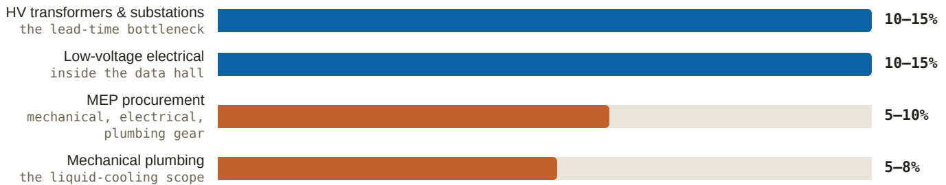
Figure 13: Where the money lands inside the fence (share of a load-center budget, %)
