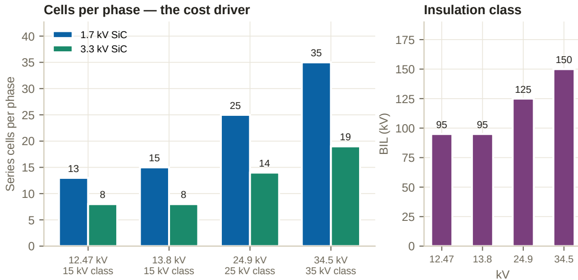
Figure M9 — What the 35 kV class costs inside the converter. Boundary: cell counts are computed for this briefing on the primer's stated assumptions — cell DC link = 0.55 \times \text{device rating} , phase peak = V_{LL} \cdot \sqrt{2}/\sqrt{3} \times 1.10 grid overvoltage, plus one redundant cell per phase [PRIMER fig.5]. Real designs vary the derating and the redundancy, so the ratios between classes are what matter and not the absolute counts. BIL is the ANSI C84.1 equipment class, not a vendor figure.
