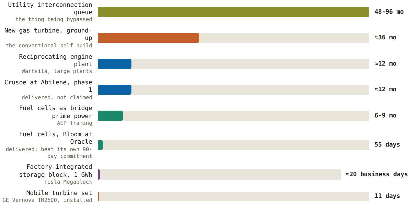
Figure 7: Time to power by route (months from decision to energized; vendor claims and delivered projects)
