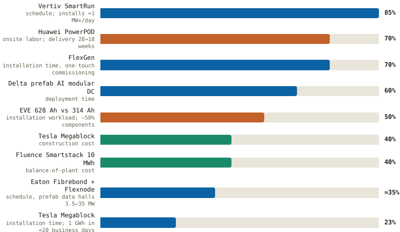
Figure 12: Prefabrication's claimed compression versus conventional stick-build (% reduction; vendor claims, differing bases)
