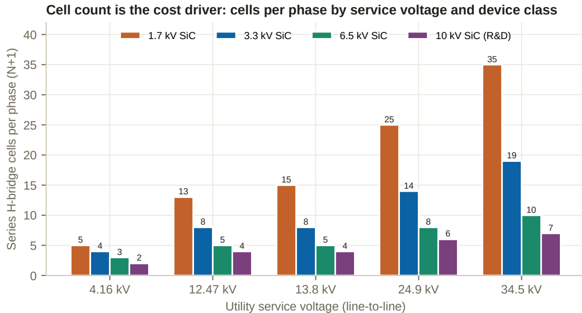
Figure 5 — Cell count is the cost driver: series cells per phase by service voltage and SiC device class. Estimate computed for this primer: cell DC link = 0.55 \times device rating (the customary derating for cosmic-ray failure rate and switching overshoot), phase peak = V_{LL} \cdot \sqrt{2}/\sqrt{3} \times 1.10 grid overvoltage, plus one redundant cell per phase. Each cell is a complete converter with its own capacitor bank, medium-frequency transformer and secondary bridge, so the count multiplies parts, gate drivers, sensors and failure points. Real designs vary the derating and redundancy; the ratios between bars are what matter.
