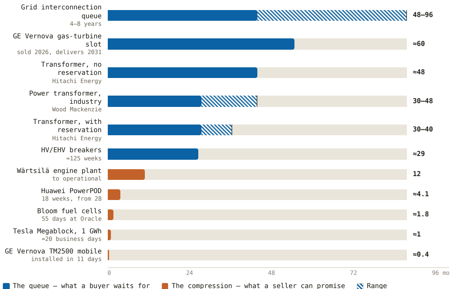
Figure 3: The master clock – queue times versus what compression products promise (months)
