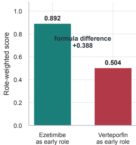
A Same profiles, exchanged roles
