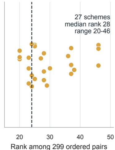
C Weight-scheme sensitivity
