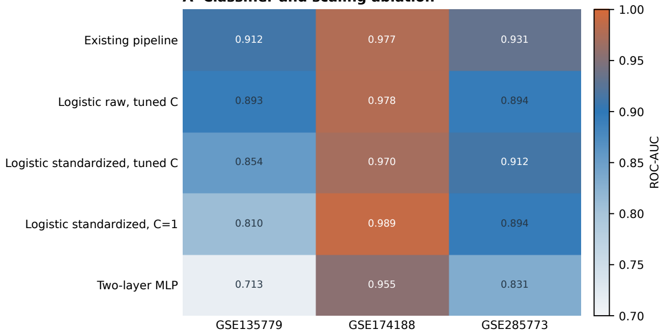
A Classifier and scaling ablation
