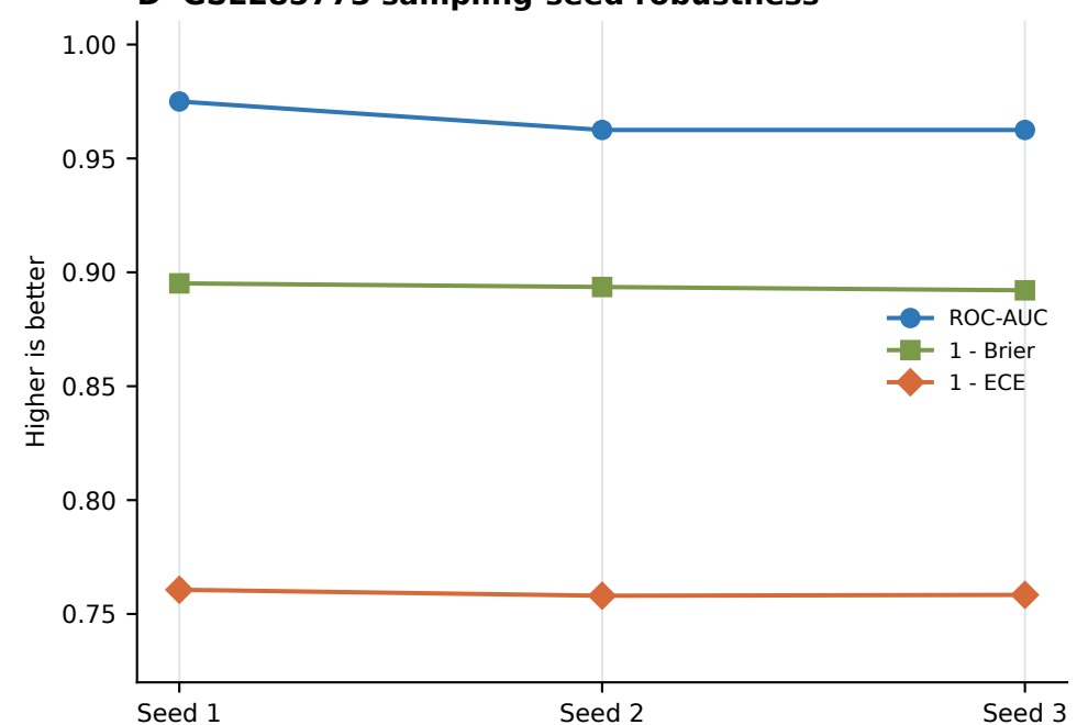
D GSE285773 sampling-seed robustness
