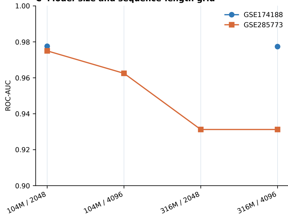
C Model-size and sequence-length grid
