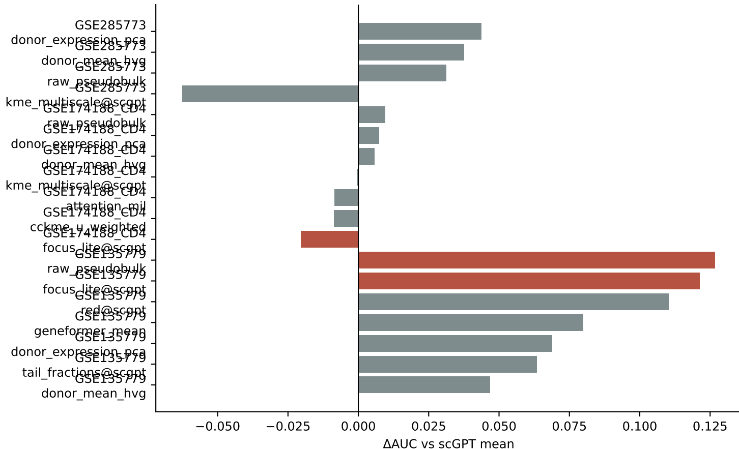
Paired donor-bootstrap method differences
