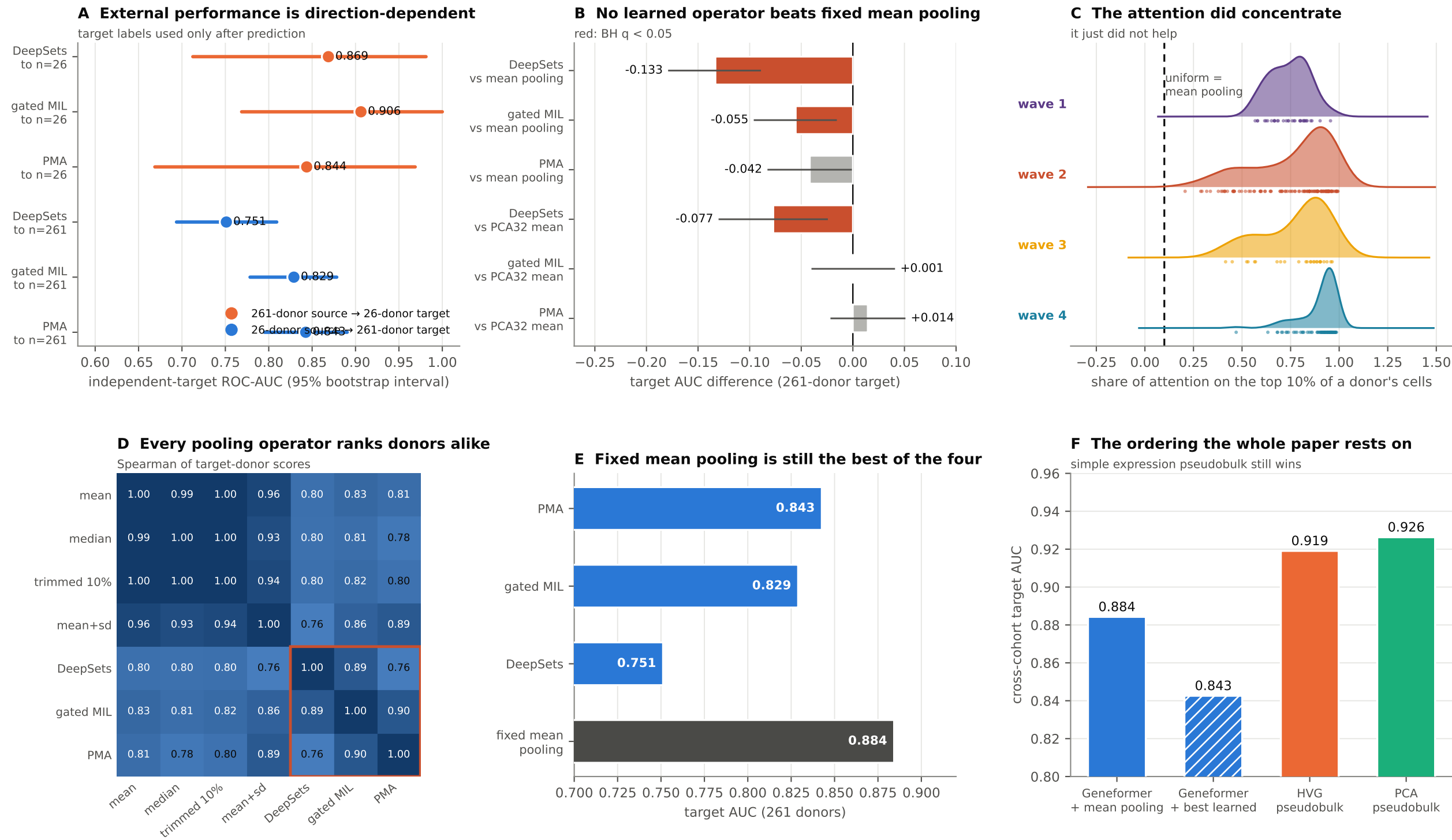
Figure 6 Learned pooling does not rescue the frozen representation
