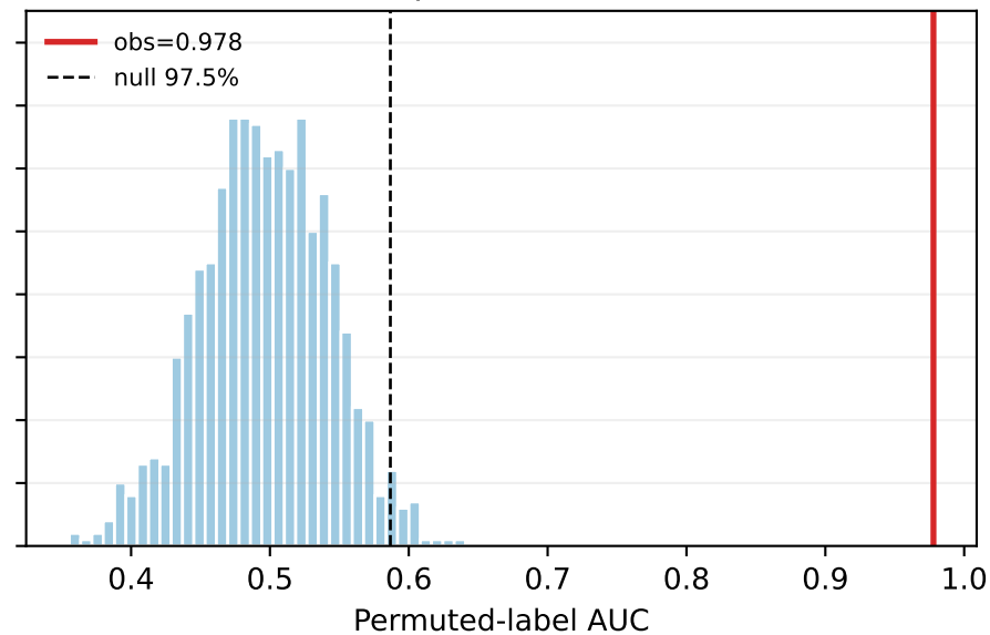
kme_multiscale@scgpt p=0.0010
