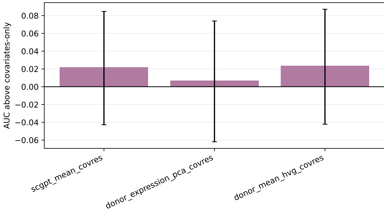
P8.6 residualized methods vs covariates-only
