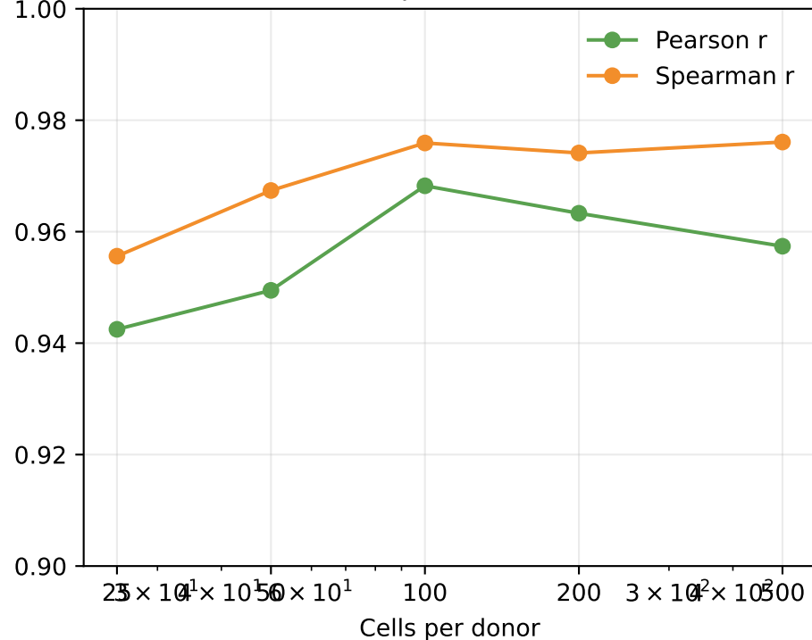
KME vs scGPT prediction correlation
