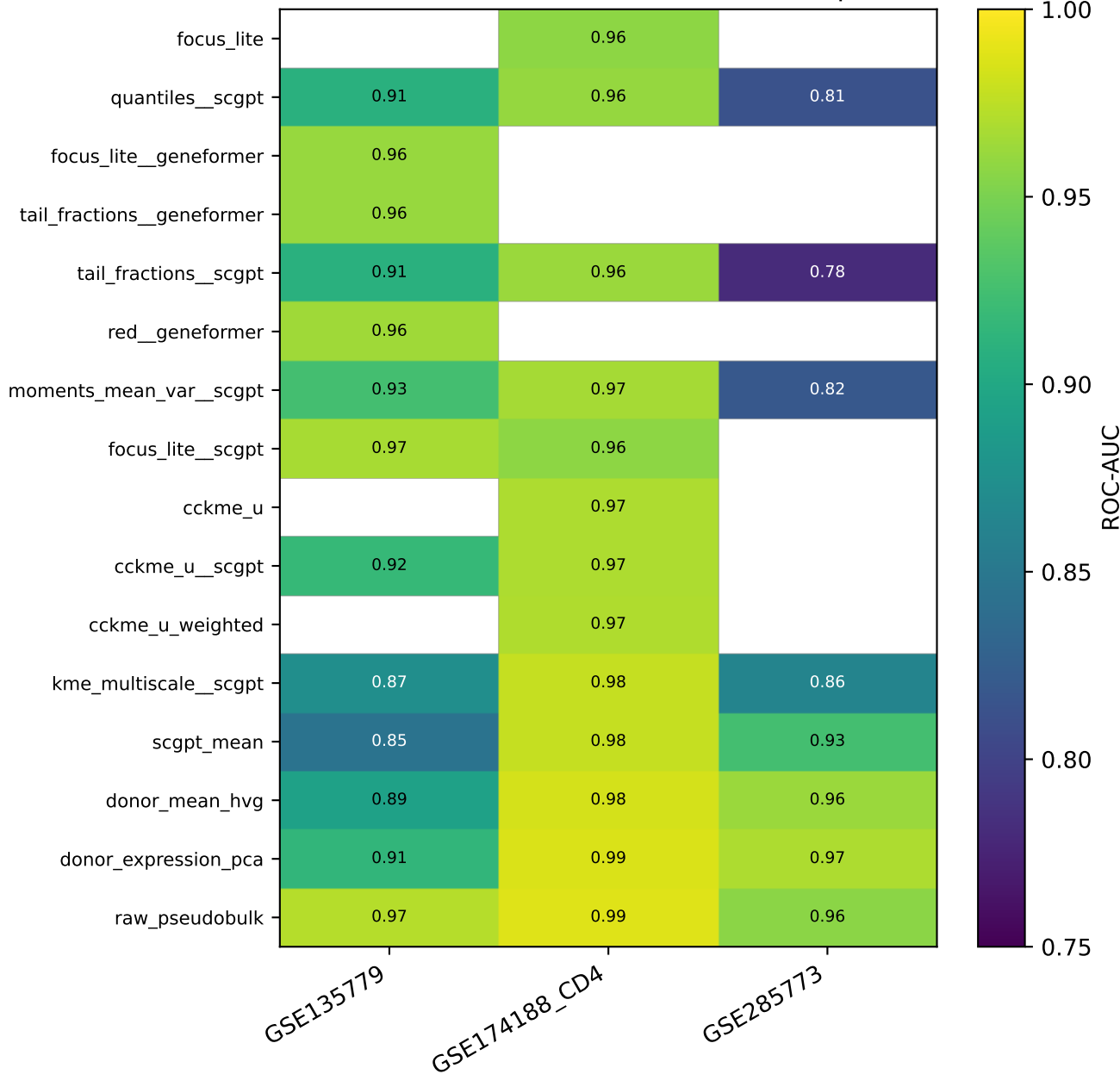
Three-cohort method AUC heatmap
