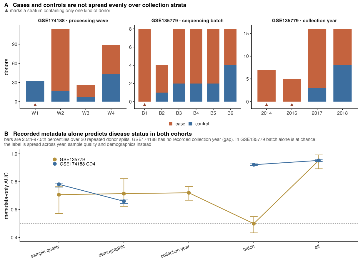
Figure 4. Collection strata and disease status in the two lupus cohorts. (A) Donors per collection stratum, split by case and control, for processing wave in GSE174188 and for sequencing batch and collection year in GSE135779. A triangle marks a stratum holding only one kind of donor; such strata cannot be permuted within, and cannot be restricted to. (B) Cross-validated AUC for predicting the diagnosis from recorded metadata alone, by variable group, with 2.5th-97.5th percentiles over 20 repeated donor splits. GSE174188 has no recorded collection year, so its line is broken there. In GSE135779 batch alone sits at chance (0.499) while the other groups do not, so the association runs through collection year, sample quality and demographics rather than through batch.
