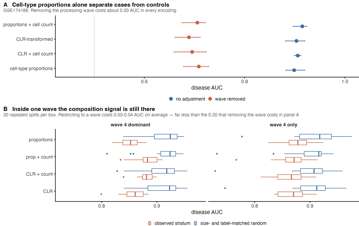
1124 Figure S5. Cell-type composition reproduces the whole pattern. (A) Diagnosis AUC in 1125 GSE174188 from four cell-type fractions alone, under four encodings, before and after removing 1126 the processing wave. Removing the wave costs about 0.20 AUC in every encoding. (B) The same 1127 encodings restricted to the dominant wave and to the pure wave, each against a size- and label- 1128 matched random donor subset, 20 repeated splits per box. Restriction costs 0.03 to 0.04 AUC on 1129 average - far less than removal costs in (A). A four-number biological summary shows the same 1130 behaviour as a 1152-dimensional foundation-model embedding, which places the problem in the 1131 cohort rather than in the embedding.
