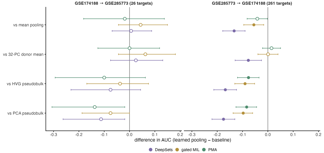
Figure S6. Learned pooling never beats averaging the cells. Paired differences in AUC between three learned pooling methods (DeepSets, gated-attention multiple-instance learning, pooling by multi-head attention) and four baselines, in both transfer directions, with paired DeLong intervals. Filled points are significant after Benjamini-Hochberg adjustment; every significant difference is negative.
