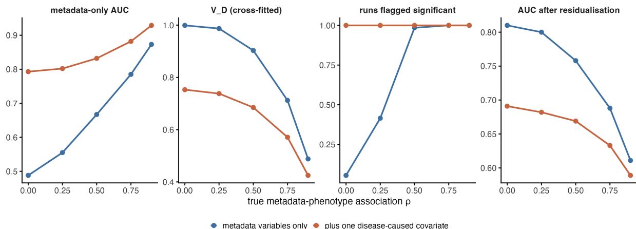
Figure S1. Admitting one disease-caused covariate produces a spurious metadata association. Metadata-only AUC, V_D, the fraction of runs flagged significant, and residualisation loss, with and without a severity variable added to the metadata matrix, across five levels of true metadata-phenotype association. At \rho = 0 , where metadata and phenotype are unrelated by construction, admitting the covariate raises metadata-only AUC from 0.488 to 0.793 and flags the cohort in 100% of runs against 5.5% without it.
