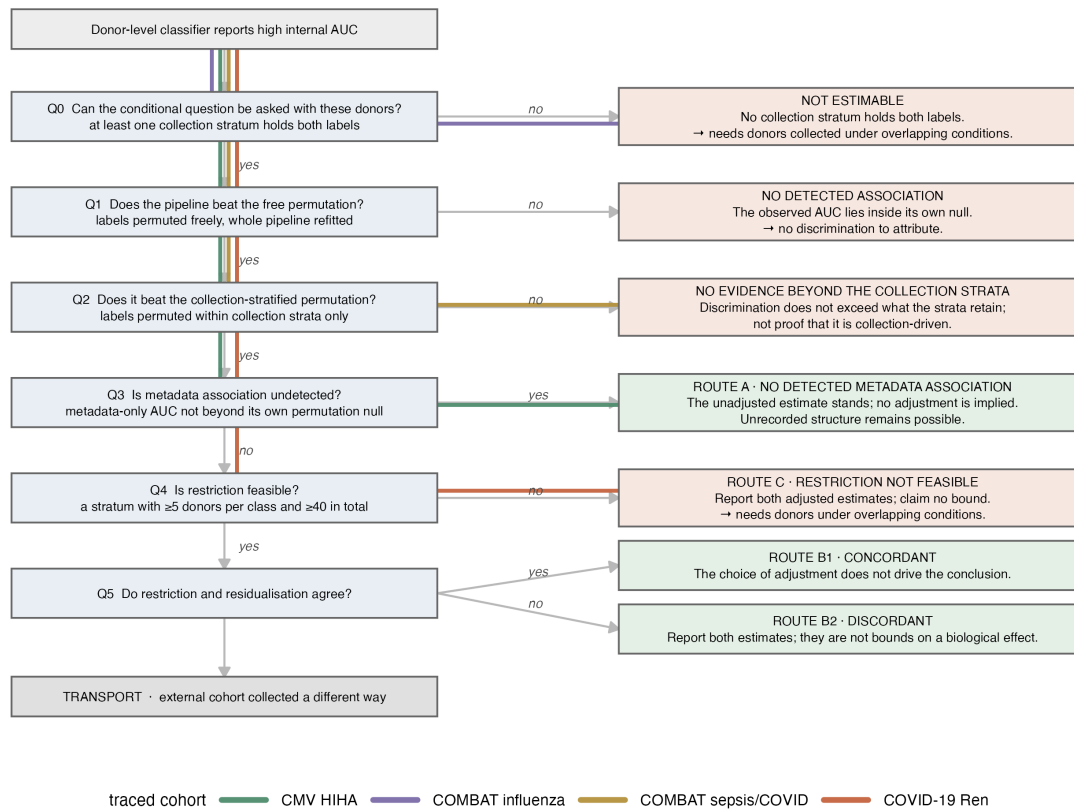
Figure 8. A decision tree for applying the checks. The feasibility question comes first (Q0): a comparison is set aside when no collection stratum holds both labels, so that no conditioned estimate can be formed. The permutation step is then split into two questions that state different nulls - the free test (Q1) and the collection-stratified test (Q2). Q3 reads the metadata-only AUC against its own permutation null rather than against a fixed cut-point; a null result there reports that no collection association was detected and leaves the unadjusted estimate standing, and does not recommend an adjustment. Q4 requires restriction to be feasible - some stratum with at least five donors of each class and at least 40 in total - so each comparison has one output; where it is not, the comparison takes Route C. Every terminal box states what can be estimated and what is still missing, not a remedy to apply. Coloured paths trace four real comparisons. The strata are the ones the collection-stratified permutation uses, not a separate definition.
