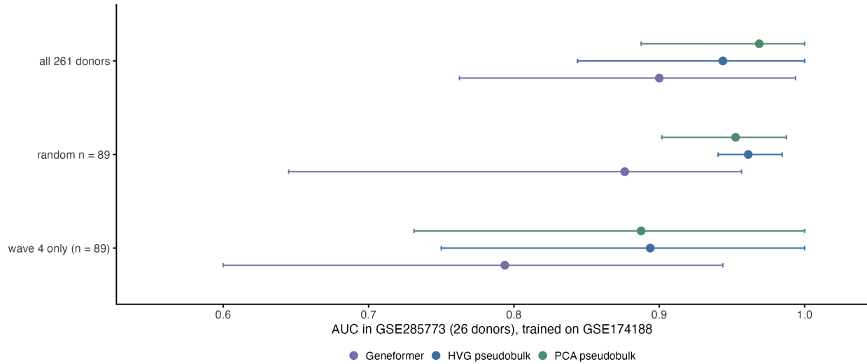
Figure 7. Restricting the training set to one processing wave does not improve transfer.
