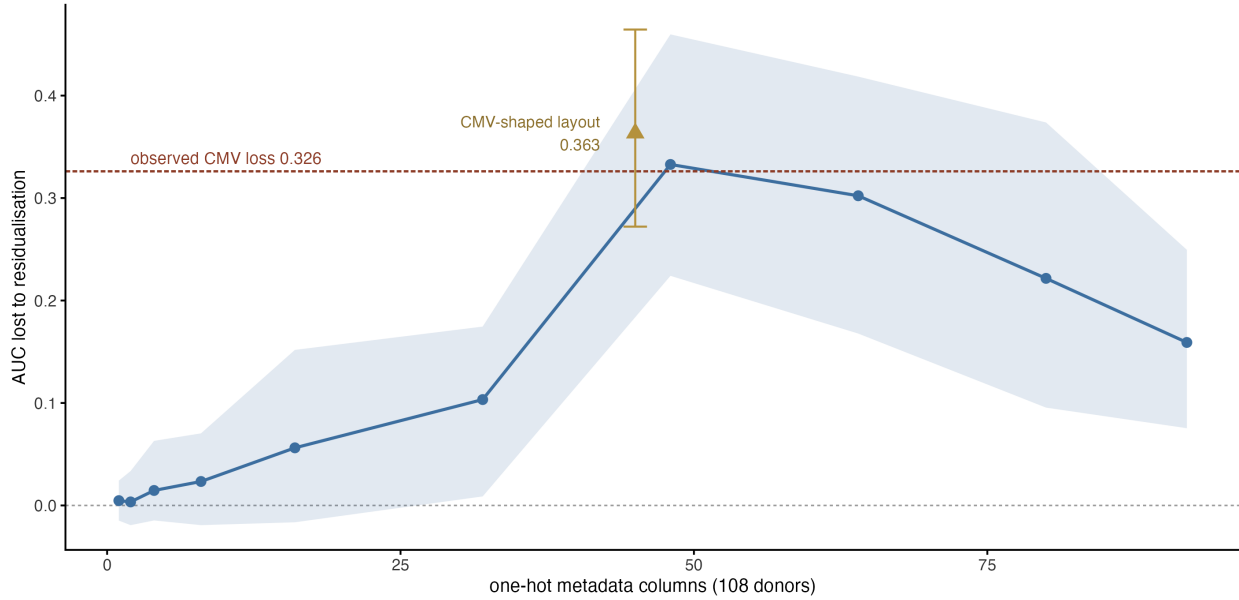
1114 Figure S4. Residualisation loss with no metadata-phenotype association present. AUC 1115 lost to fold-contained ridge residualisation in simulated cohorts where the metadata matrix is 1116 independent of the phenotype by construction, against the width of that matrix, at 108 donors. 1117 The unadjusted and residualised arms share folds, feature filter, standardiser, PCA and classifier 1118 and differ only in the adjustment. The biological effect is calibrated so the unadjusted AUC lands 1119 near 0.90. The ribbon is the 2.5th-97.5th percentile over 60 draws. The triangle reuses the level 1120 sizes of the real CMV batch-by-pool crossing, which is far more ragged than equal blocks; it loses 1121 0.363 on average. The dashed line marks the 0.326 observed in that comparison, which falls inside 1122 the triangle's interval.
