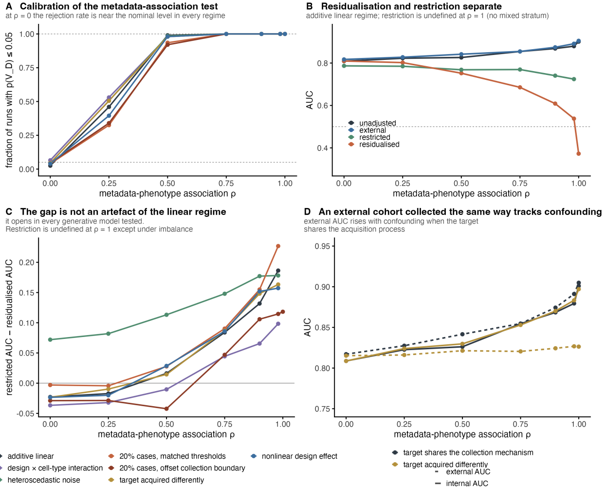
Figure 3. Simulation across seven data-generating regimes. 19,600 simulated cohorts (200 donors, 100 features): seven regimes \times seven levels of metadata-phenotype association \rho \times two label types \times 200 replicates. (A) Fraction of runs with p(V\_D) \leq 0.05 , binary labels. At \rho = 0 this is 0.025 to 0.065 across regimes, bracketing the nominal 0.05. (B) Unadjusted, external, restricted and residualised AUC against \rho in the additive linear regime. Restriction is undefined at \rho = 1 because no stratum holds both labels. (C) Restricted minus residualised AUC for all seven regimes. The gap opens in every one. It is blunted in the imbalanced-offset regime, where the collection boundary and the phenotype threshold sit at different quantiles, and not in the imbalanced regime, where the case rate is the same 20% but the two are matched (Section 4.3). (D) Internal (solid) and external (dashed) AUC when the target shares the source’s collection mechanism versus when
