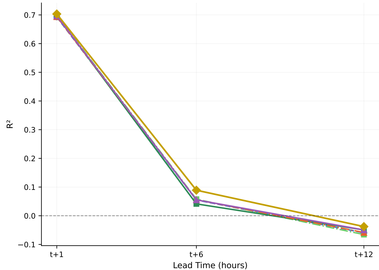
(b) R^2 Score
