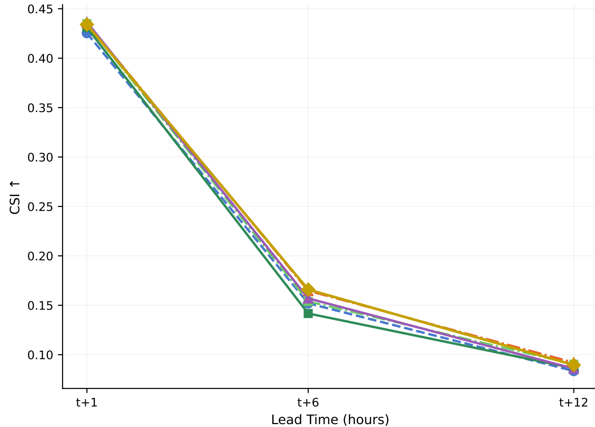
(a) CSI (Critical Success Index)
