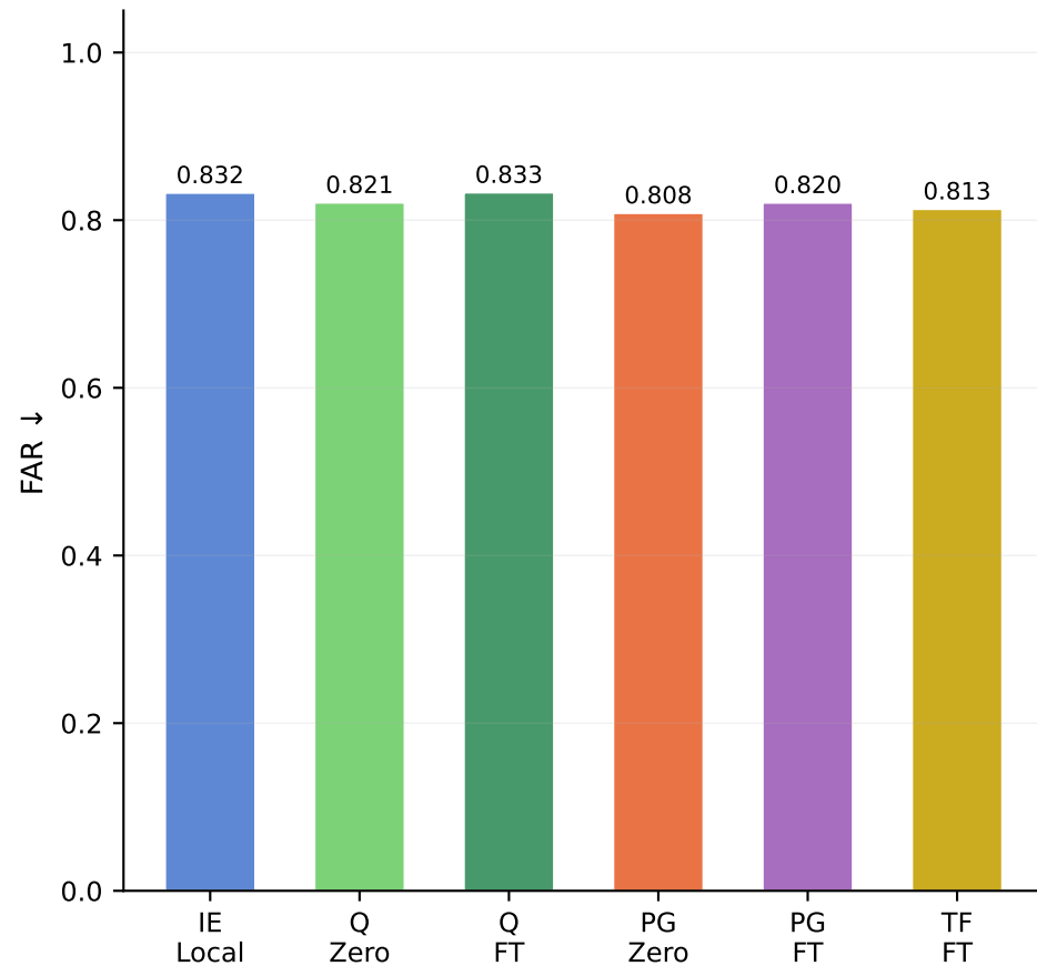
Lead Time t+6
