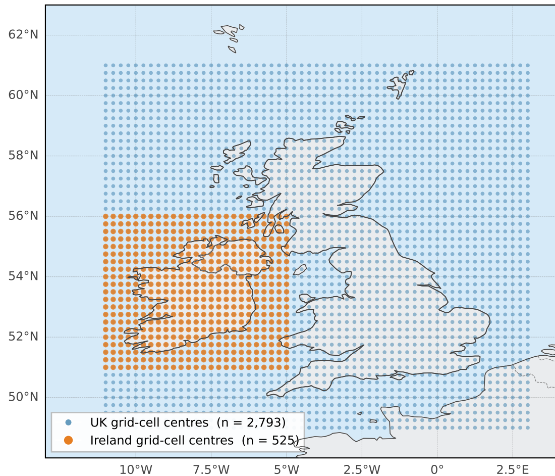
(b) ERA5 grid-cell centres
