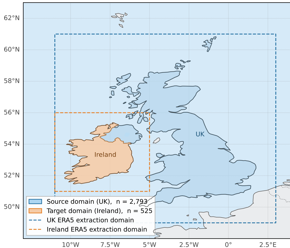
(a) Study area overview
