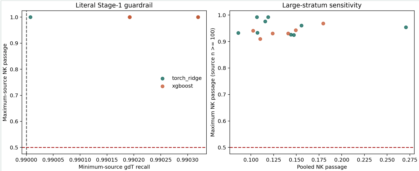
Literal and sample-size-aware Stage-1 diagnostics.
