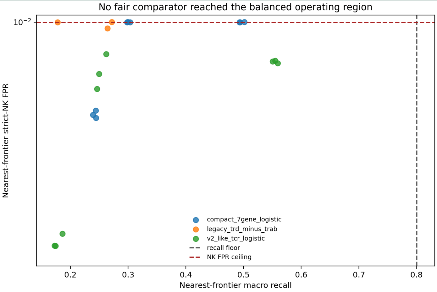
Balanced comparator near-miss operating points.
