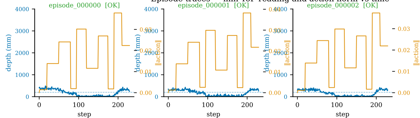
Episode traces — min ToF reading and action norm vs time
