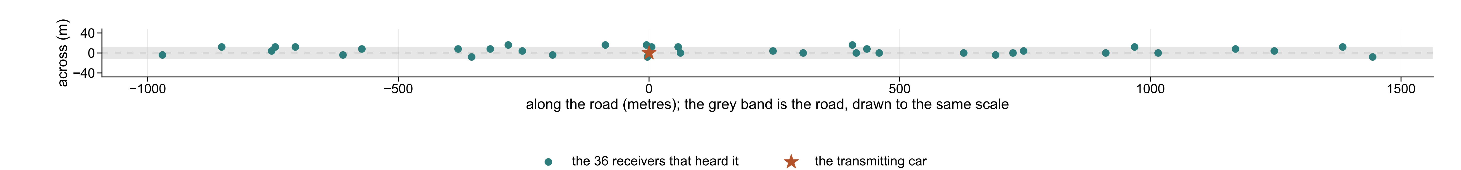
Figure 3. The receivers that heard one car span 2,414 m along the road and 24 m across it. They measure distance along the road well and across it poorly, so an attacker who knows this lies sideways.
