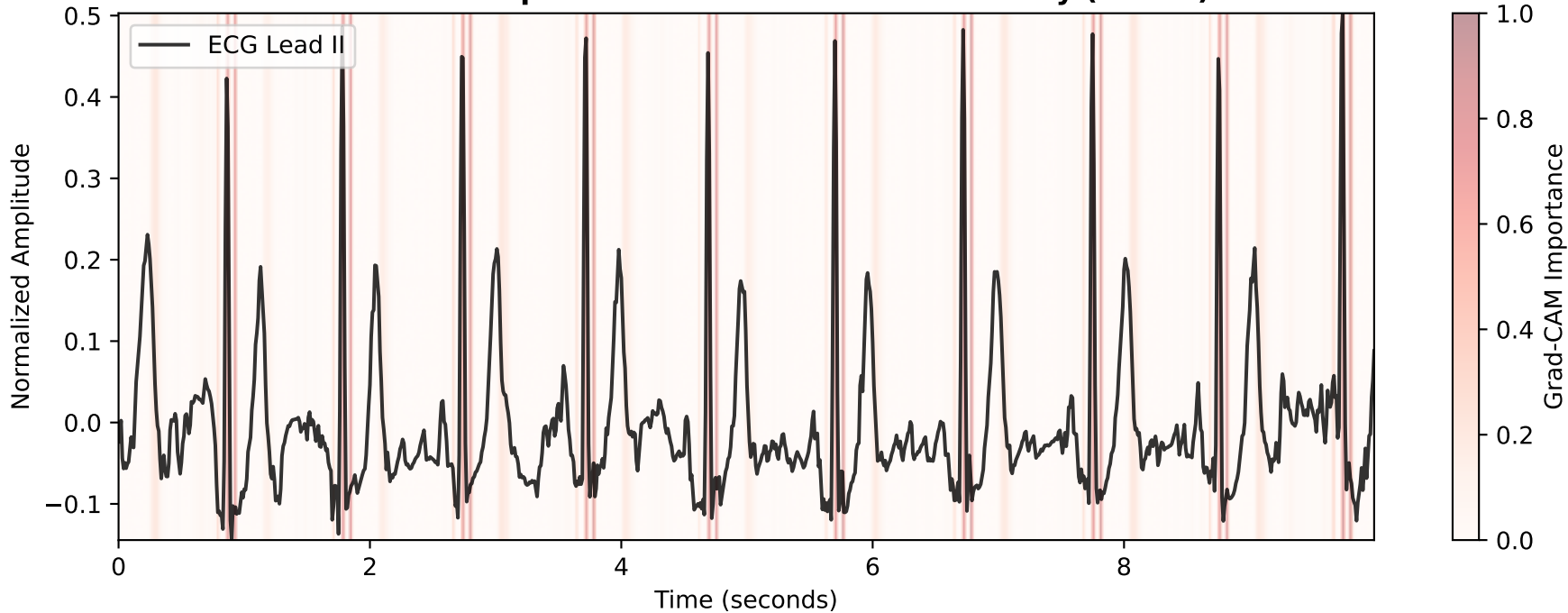
Grad-CAM Temporal Localization: Lead II Overlay (NORM)
