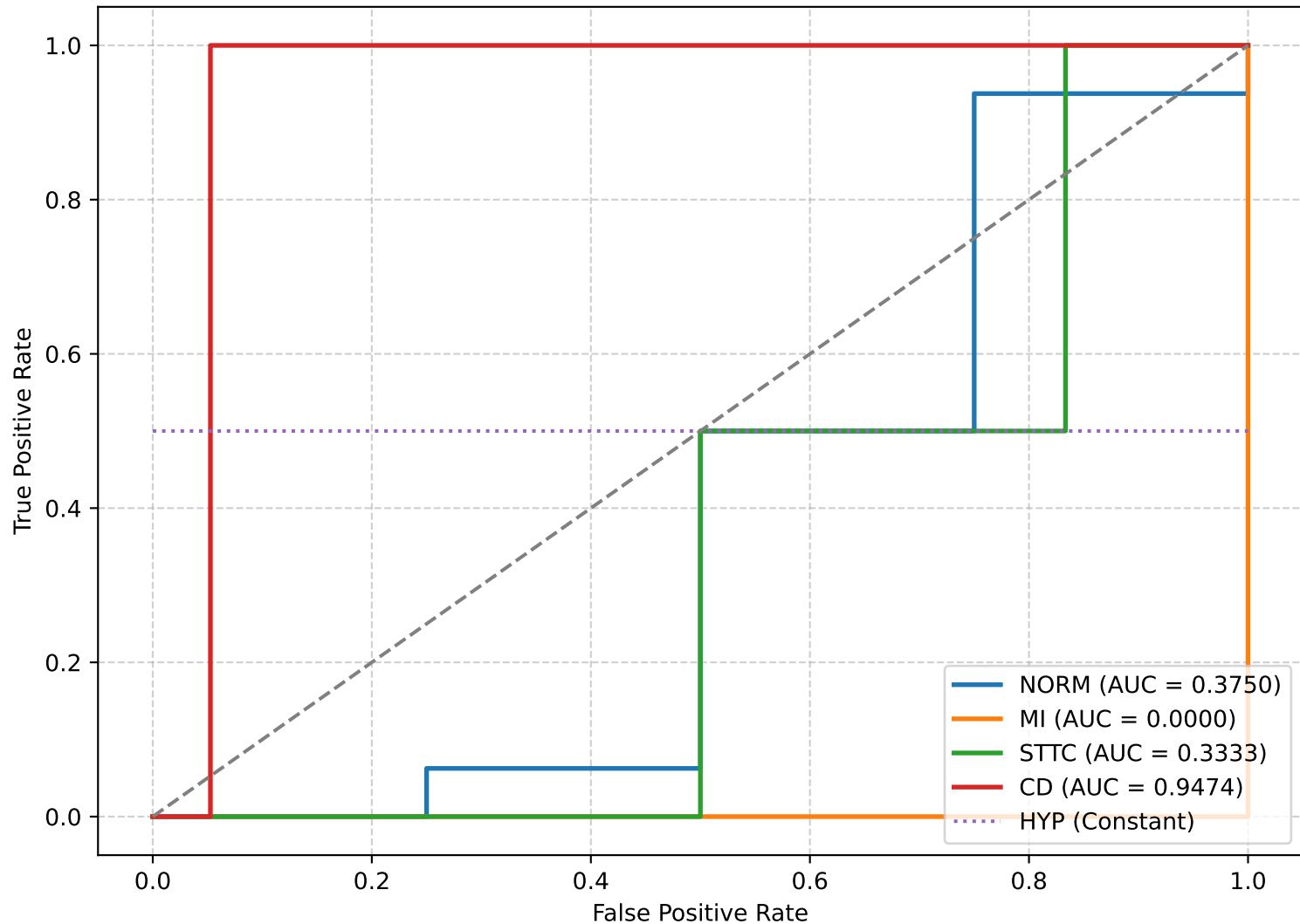
ROC Curves - Best Late-Fusion Model (Feature_Attention)
