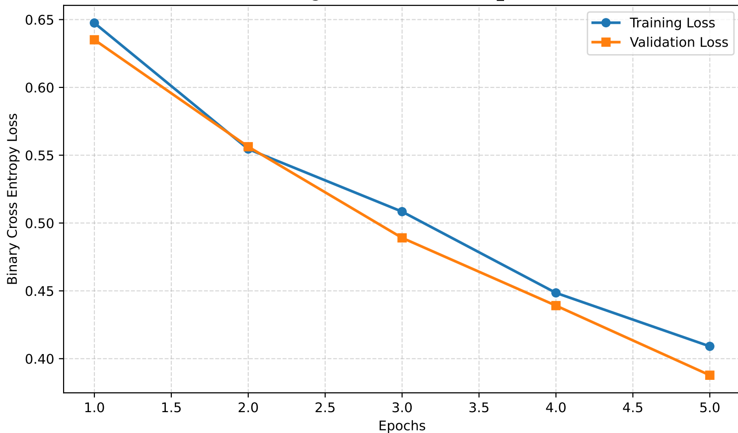
Model Loss Convergence Curves (Feature_Attention Fusion)
