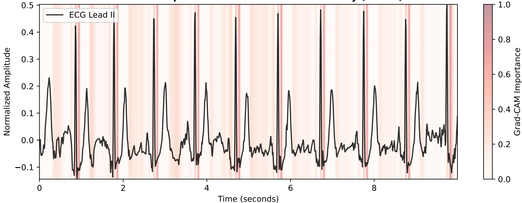
Grad-CAM Temporal Localization: Lead II Overlay (NORM)
