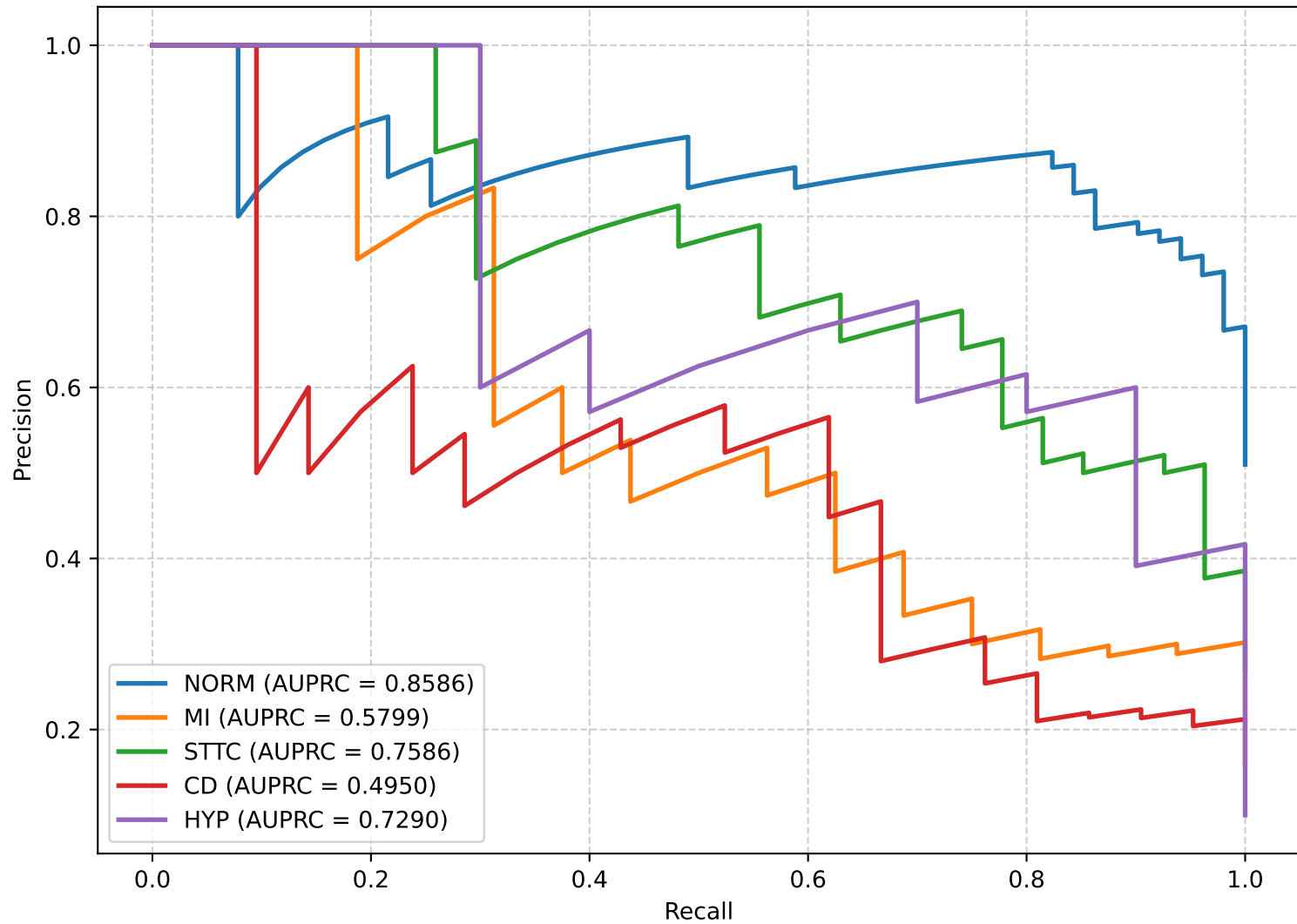
Precision-Recall Curves - Feature_Attention Fusion
