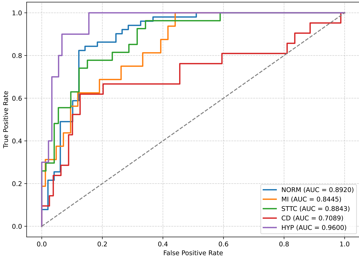
ROC Curves - Best Late-Fusion Model (Feature_Attention)
