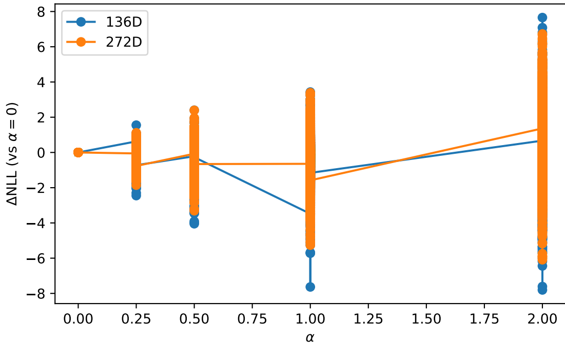
Predictive usefulness: 136D vs 272D (real)
