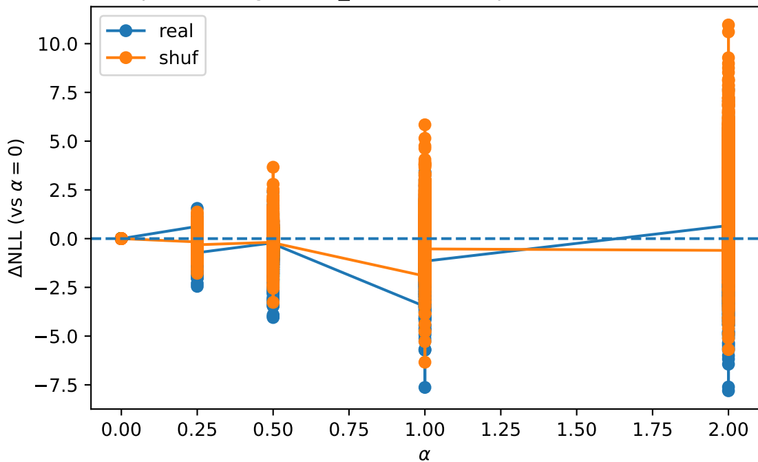
Alpha scaling (brain_dim=136) — predictive usefulness
