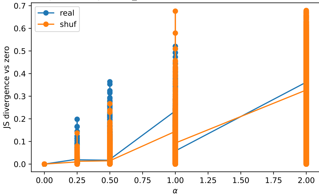
Alpha scaling (brain_dim=136) — distribution deformation
