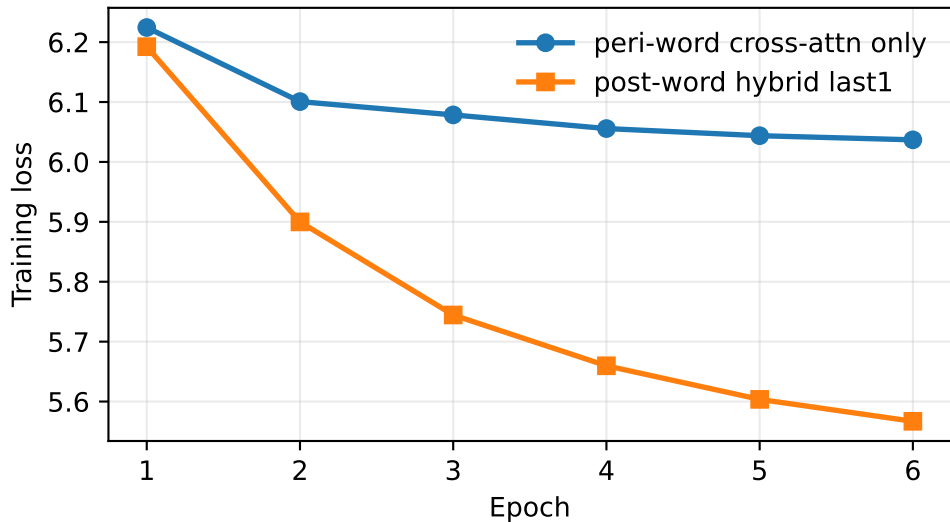
MEG-T5 diagnostic training loss
