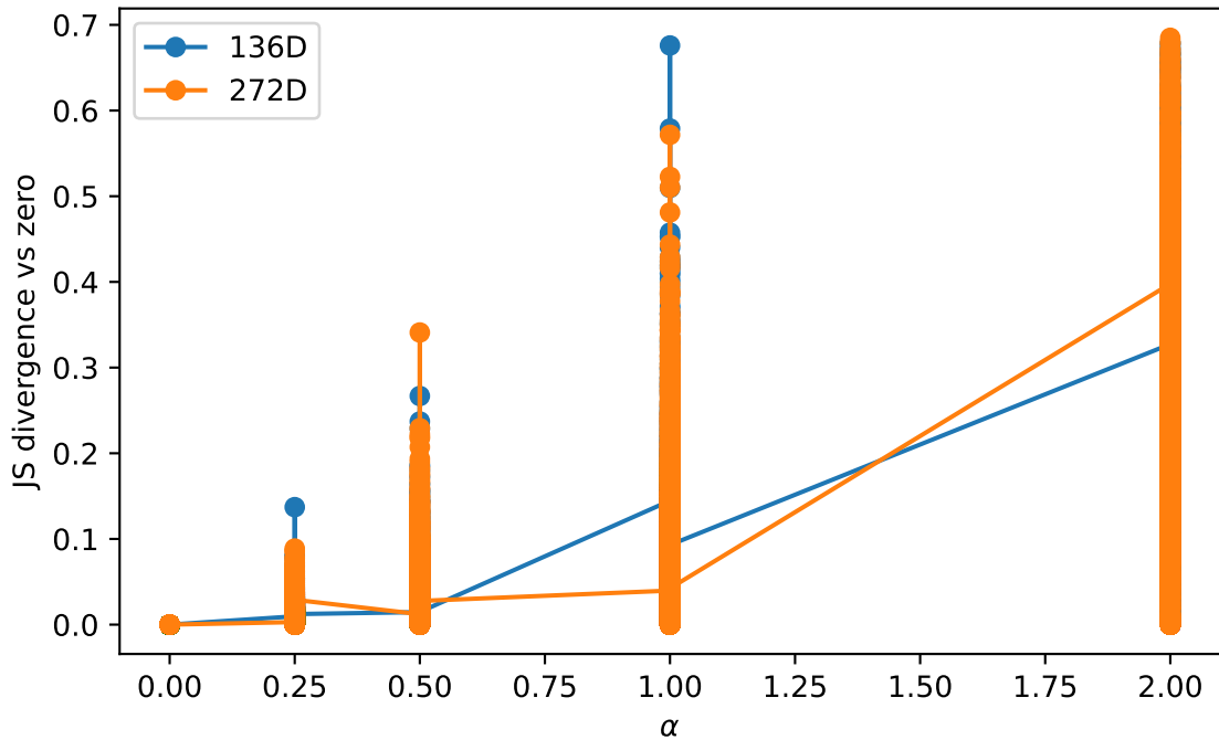
Distribution deformation: 136D vs 272D (shuf)
