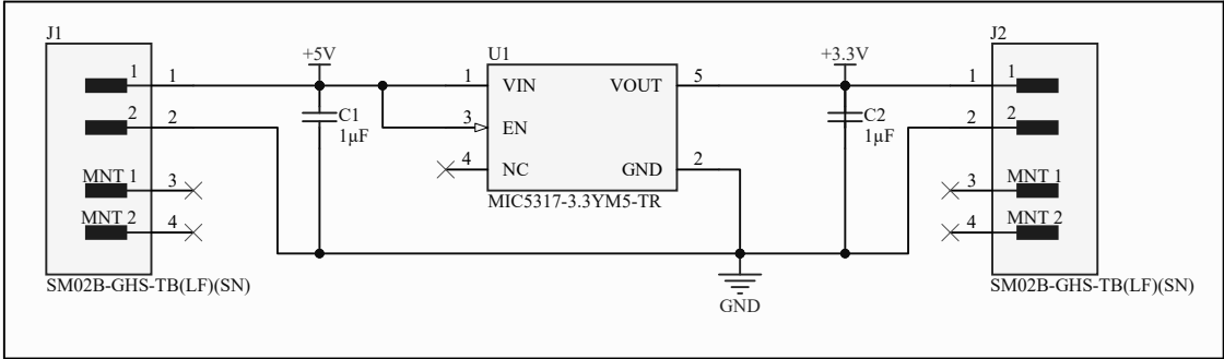
5V to 3.3V Voltage Regulator
